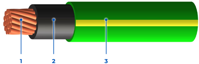
Safe-T-Stripes Conductor 1 – Strand Bare (ASTM B8) Annealed Copper Conductors
